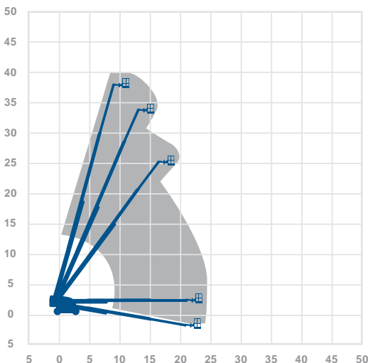
Working Envelope
