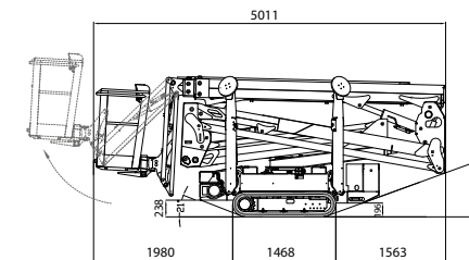
Side elevation
