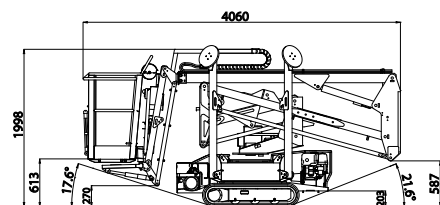
Side elevation
